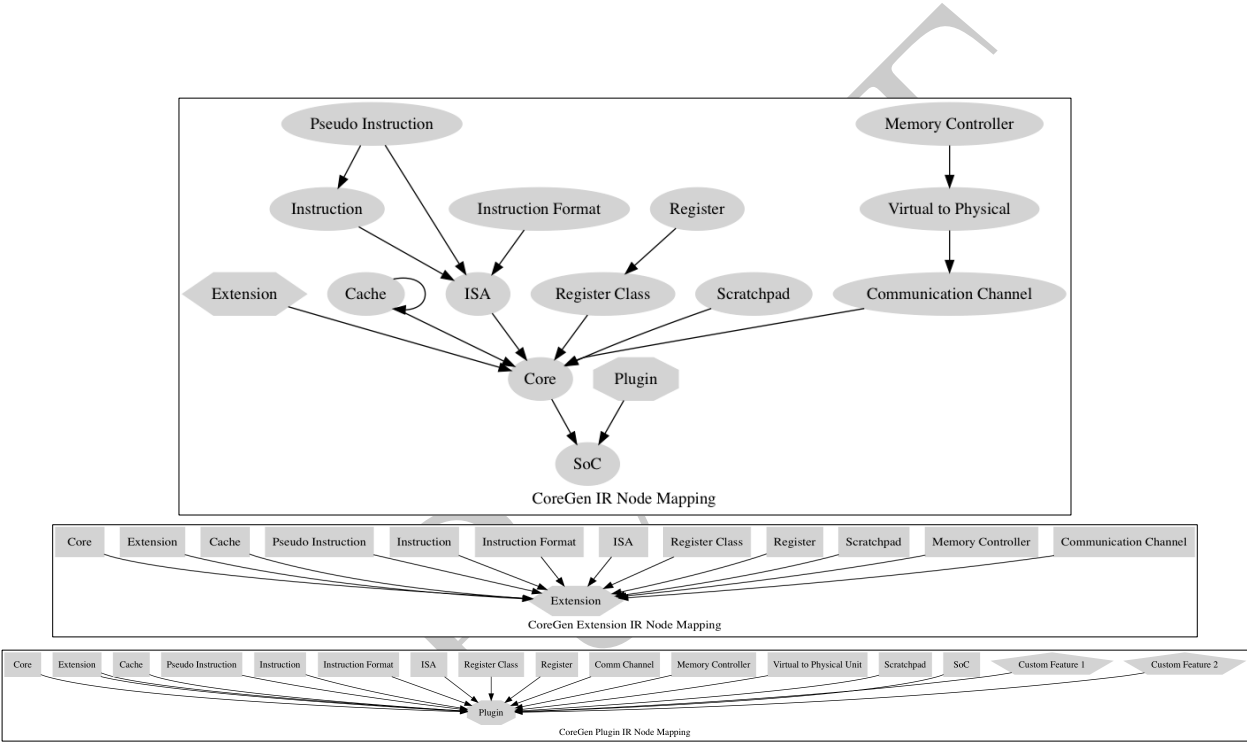
Figure 1: CoreGen IR Node Hierarchy
